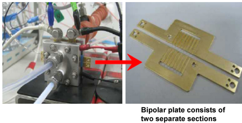
Fig. 4. The 2 cm 2 active area PEFCs for cross-sectional observations of the GDL and MEA, here the bipolar plates consist of two separate sections.
