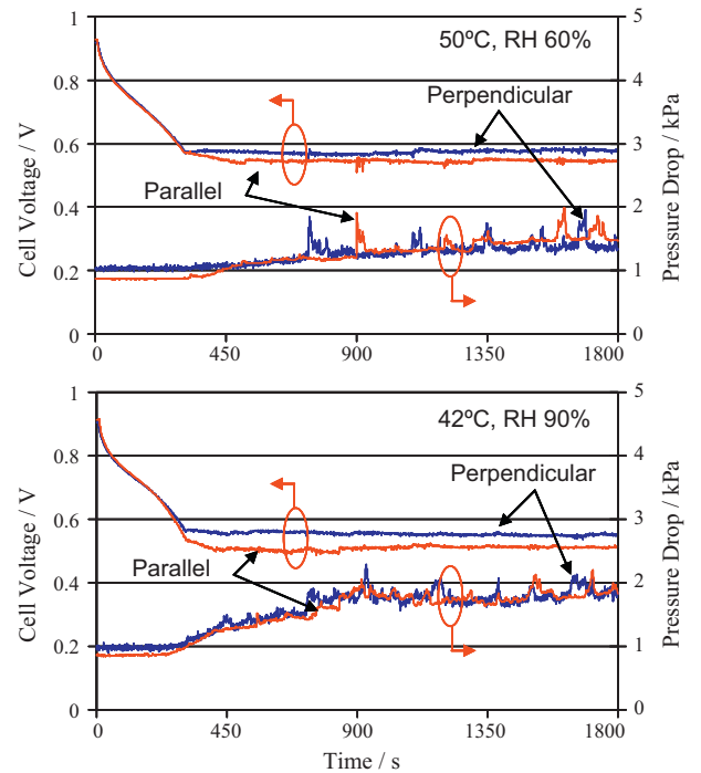
Fig. 6. Voltage changes for the two types of anisotropic GDL, perpendicular and parallel, at different humidity conditions (0.5 A cm -2 ).
