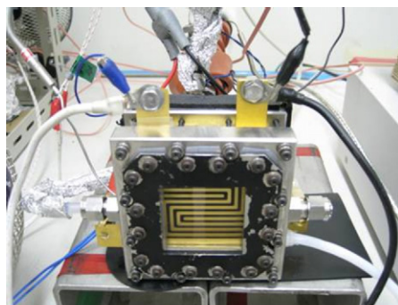
Fig. 2. Experimental apparatus for visual observations and a schematic illustration of a 25 cm 2 active area PEFCs.
