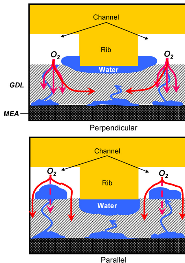
Fig. 10. Experimentally suggested images of liquid water distribution and gas flow paths in the GDL: perpendicular fibers (top) and parallel fibers (bottom).
