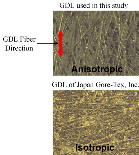
Fig. 1. Anisotropic and isotropic GDLs.
