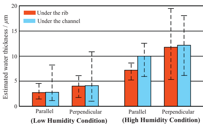
Fig. 16. Estimated average thickness of water distributions at the MEA/MPL interface in the perpendicular and the parallel cells. The maximum and minimum values are shown as the error bars.
