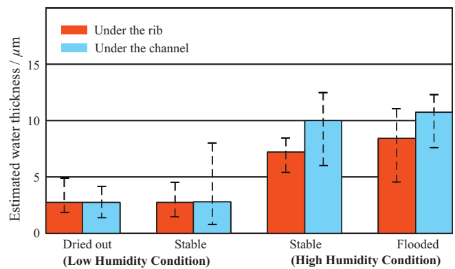
Fig. 14. Estimated average thickness of water at MEA/MPL interface in the parallel cells. The maximum and minimum values are shown as the error bars.
