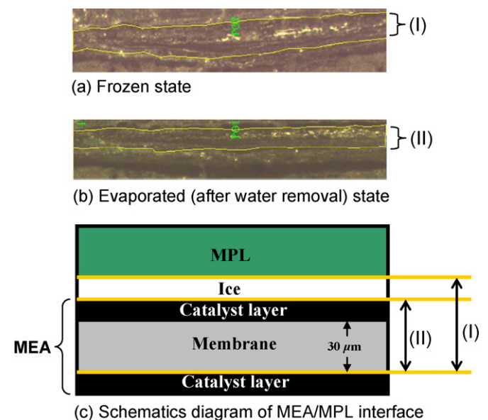
Fig. 12. The cross-sectional view of the MEA/MPL interface with (a) the area (within the yellow lines) of the catalyst and membrane including the ice at the frozen state, and (b) the area (within the yellow lines) of the same layers after water evaporation (please ignore the green character “PG” which is created automatically in software, Image Pro.), (c) schematic diagram of the MEA/MPL interface with the reference lines (yellow lines) to measure the areas expressed in (a) and (b). (For interpretation of the references to color in this figure legend, the reader is referred to the web version of the article.)
