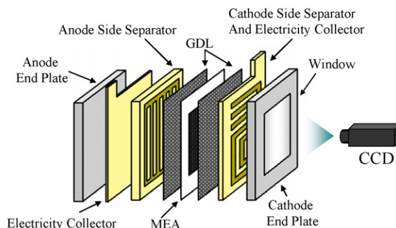
Fig. 2. Experimental apparatus for visual observations and a schematic illustration of a 25 cm 2 active area PEFCs.
