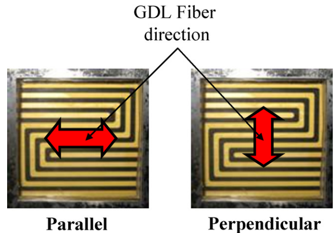
Fig. 3. Two types of configuration of the anisotropic GDLs used in this investigation, perpendicular and parallel fiber directions.
