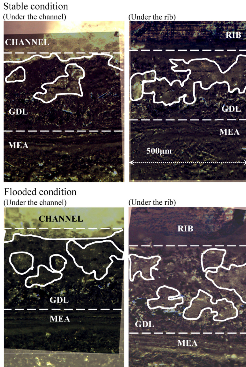
Fig. 13. The subtracted cross-sectional view of the GDL in the cathode side showing the ice distribution (within the white outlines) for the parallel fiber cell.
