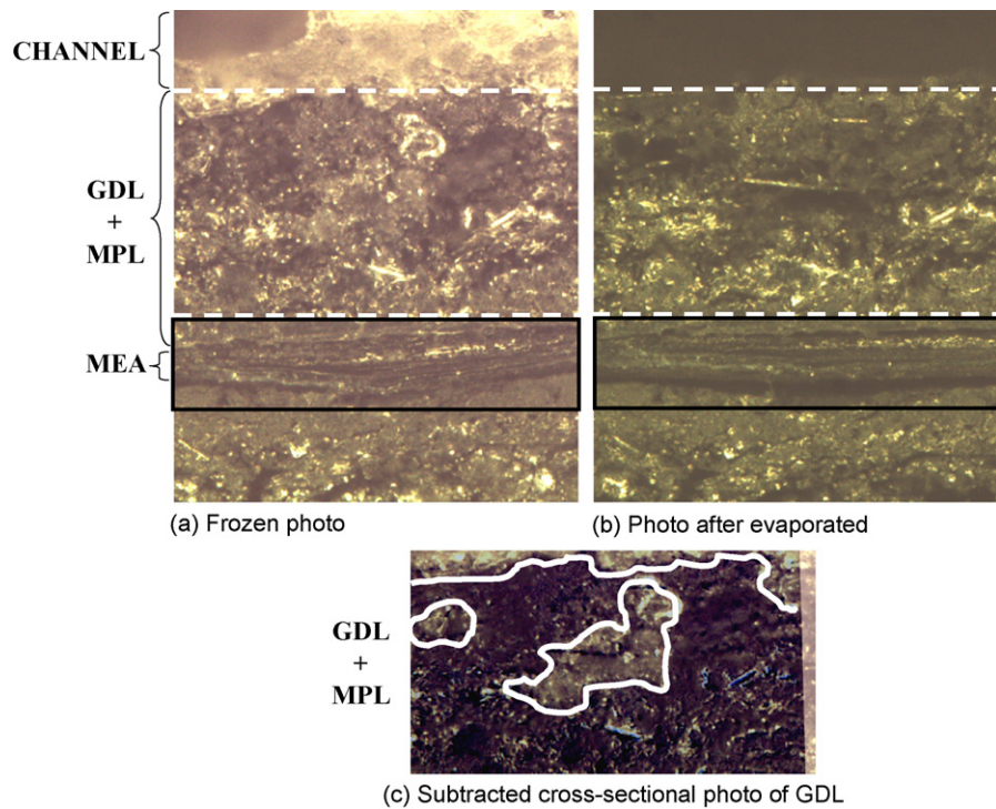
Fig. 11. Cross-sectional views of the cell at the same position of the cathode side in (a) the frozen and (b) the evaporated (after water removal) states, and (c) the subtracted cross-sectional view of the GDL with the ice distribution indicated (within white line).
