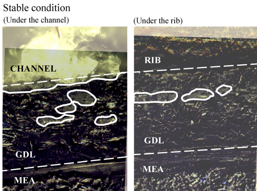
Fig. 15. Subtracted cross-sectional view of the cathode side of the cell with the ice distribution (within the white outlines) for the perpendicular fiber cell.
