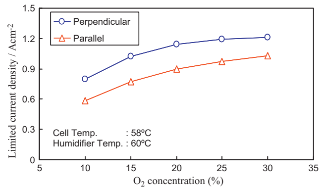
Fig. 8. Limiting current densities with various oxygen concentrations for the two types of cell here.
