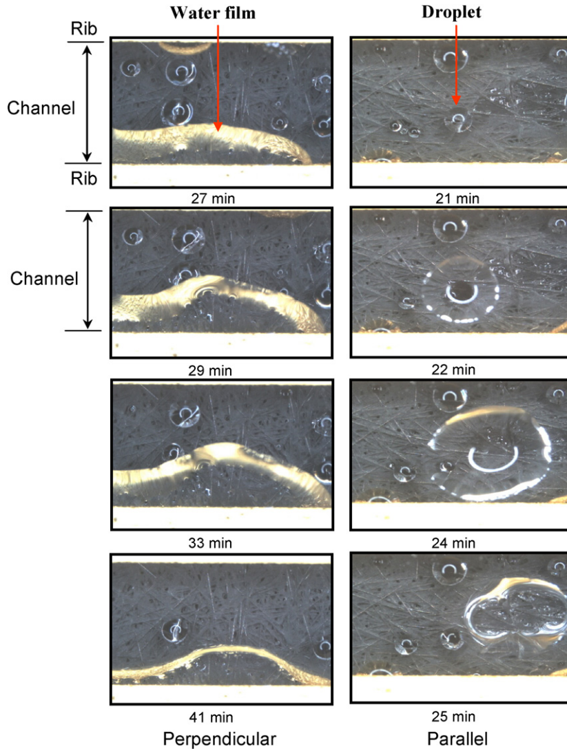
Fig. 9. Photos of the growth and changes in appearance in the liquid water film in the perpendicular cell and the changes in the size and position of a droplet in the parallel cell taken by direct visualization.
