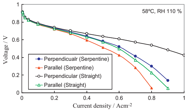
Fig. 5. Polarization curves for the two orientations of anisotropic GDL, perpendicular and parallel, with two separator types, serpentine and straight.
